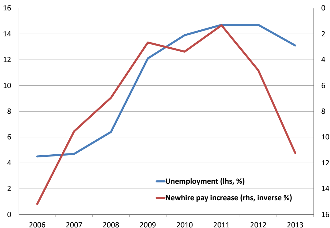
FIGURE 13. Average change in real weekly pay following a job change
