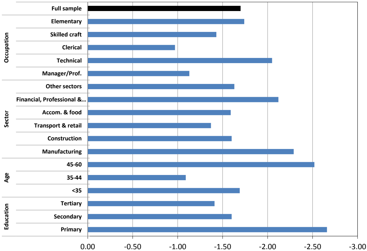
FIGURE 10. Semi-elasticities for different groups
