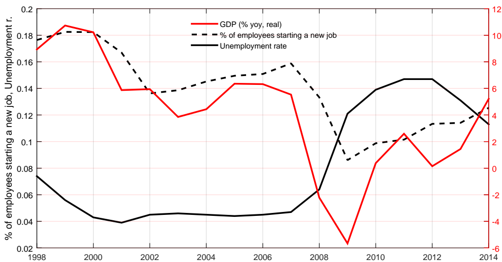
FIGURE 4. Cyclicity of job starts
